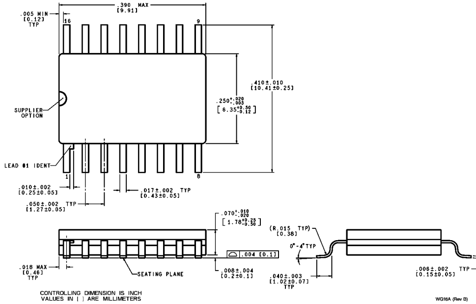
16 Lead Surface Mount Package (WG) Order Number LM2940WG5.0/883 (5962-8958701XA) See NS Package Number WG16A
